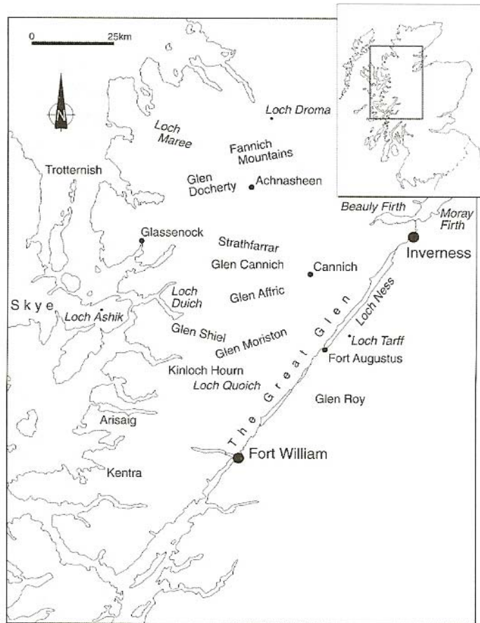
Fig. 1. The area of Glen Affric and Kintail in the NW Scottish Highlands, showing its location, relation to major towns and natural features, and key localities in the region outwith the study area.
